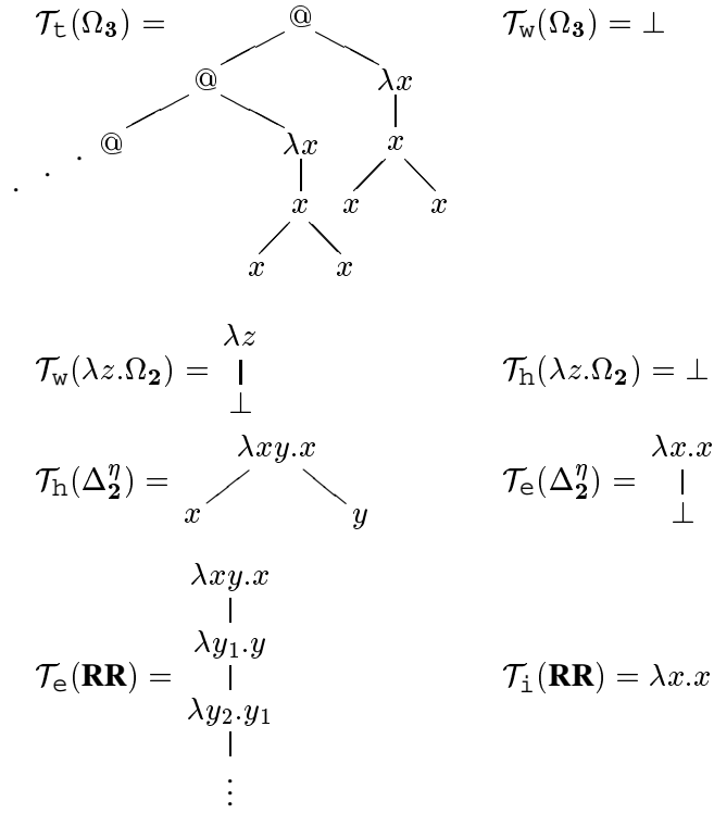
Fig. 2. Trees for Example 6
