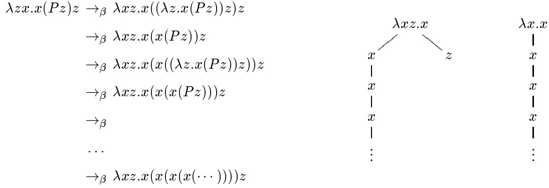
Fig. 1. Reduction path, head tree and eta tree for \lambda x z.x(Pz)z , where P \rightarrow_{\beta} \lambda z.x(Pz) .
