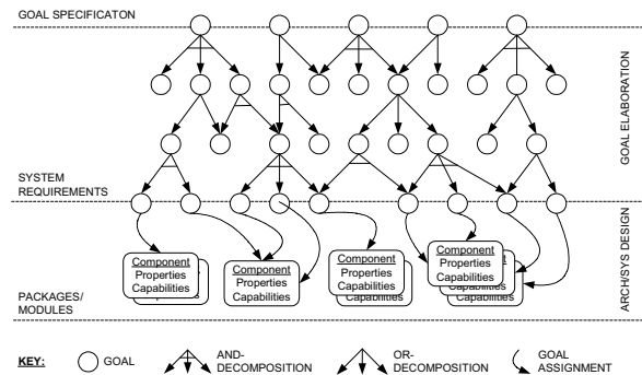
Figure 2: Goal refinement hierarchy
