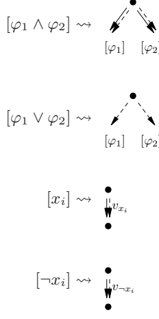
Fig. 11. Deterministic rules rewriting a QCNF formula \varphi into a specification (N_\varphi, t_\varphi)
