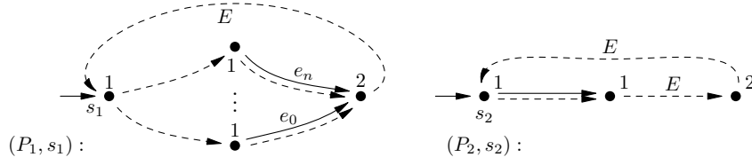
Fig. 2. Modal specifications (P_1, s_1) and (P_2, s_2) together ensuring that Player 1 can always continue playing. Assume E = \{e_0, \dots, e_n\}
