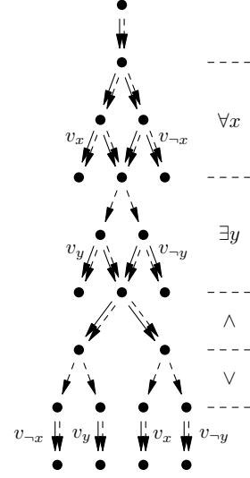
Fig. 12. Modal specification (N_\varphi, t_\varphi) for \varphi = \forall x \exists y (\neg x \vee y) \wedge (\neg y \vee x)
