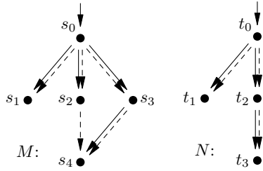
Fig. 1. Specifications (M, s_0) , (N, t_0) with I(M, s_0) = I(N, t_0) (so I(M, s_0) \subseteq I(N, t_0) ), but not (N, t_0) \prec (M, s_0)
