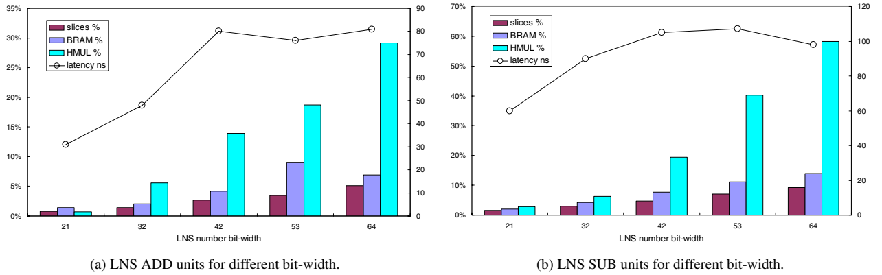
Figure 7: Hardware resource cost and latency of faithful rounding LNS arithmetic units for different bit-widths. The integer bits and fractional bits of each bit-width value are the same as the values shown in Table 1. The percentage of slices, BRAM and HMUL are calculated based on Virtex-II XC2V6000, which has 33792 slices, 144 BRAMs and HMULs.
