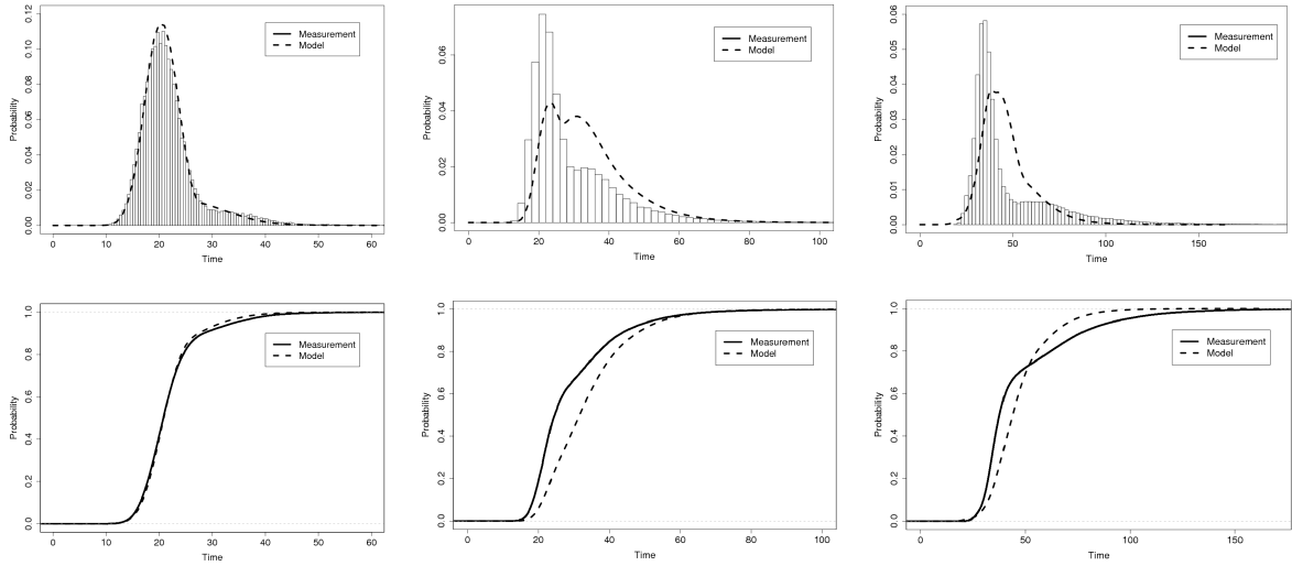
(a) 100% read requests, b = 4 , \lambda = 0.01 (b) 100% read requests, b = 6 , \lambda = 0.03 (c) 100% write requests, b = 13 , \lambda = 0.01
