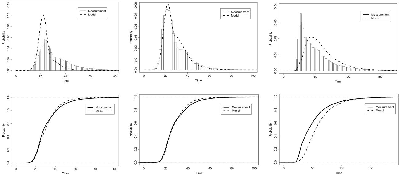
(a) 25% read requests, 75% write requests, b = 3 , \lambda = 0.03 (b) 50% read requests, 50% write requests, b = 3 , \lambda = 0.03 (c) 75% read requests, 25% write requests, b = 14 , \lambda = 0.03
