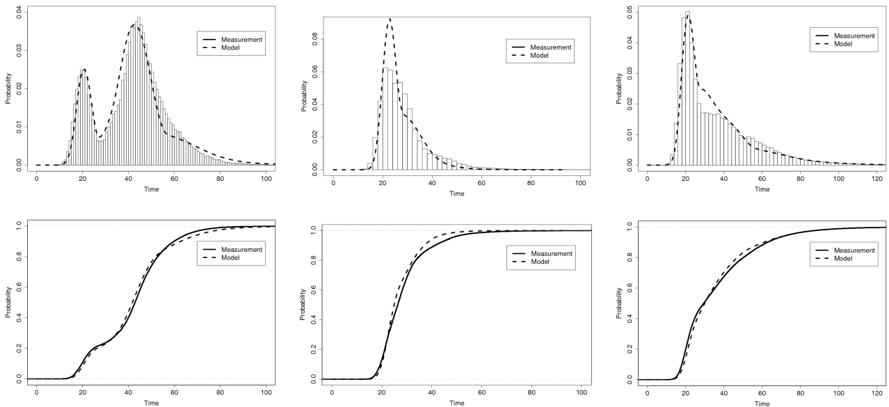
(a) 25% read requests, 75% write requests, b = 7 , \lambda = 0.01 (b) 50% read requests, 50% write requests, b = 7 , \lambda = 0.01 (c) 75% read requests, 25% write requests, b = 4 , \lambda = 0.03
