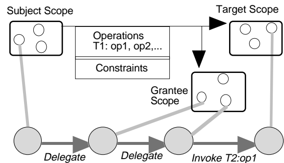
Figure 2.1: Graphical representation of an Extended Access Control Policy
